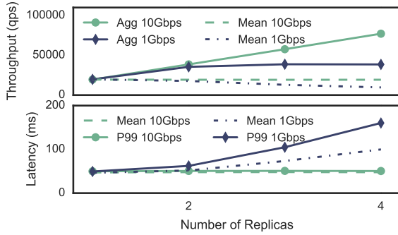
Figure 6: Scaling the Model Abstraction Layer to Remote GPUs. The solid lines refer to aggregate throughput of all the model replicas and the dashed lines refer to the per-replica average throughput. The first GPU in this cluster is located on the same machine that Clipper is running on. Subsequent GPUs are each located on separate machines on the same switch.
