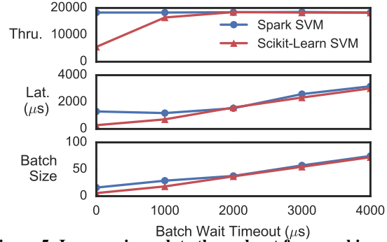
Figure 5: Increase in update throughput from caching predictions.
