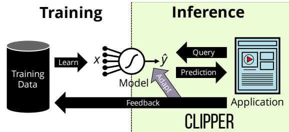
Figure 2: Machine Learning Lifecycle
