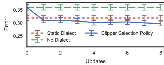
Figure 10: Personalized Corrections Accuracy of the ensemble correction policy on the speech recognition benchmark.
