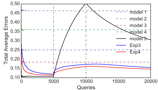
Figure 8: Behavior of Exp3 and Exp4 Under Model Failure: After 5K queries the lowest-error model suffers a failure, and after 10k queries recovers. Exp3 and Exp4 quickly compensate for the failure and achieve lower error than any static model selection.
