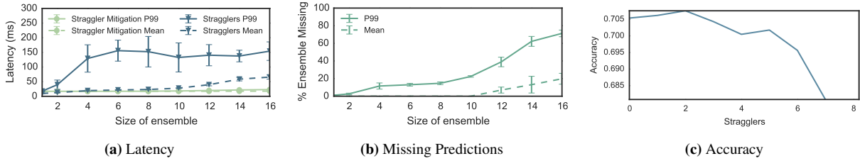
Figure 9: Increase in stragglers from bigger ensembles: The (a) latency and (b) missing predictions when using the ensemble model selection policy on SK-Learn Random Forrest models applied to MNIST. (c) The prediction accuracy of the TIMIT speech recognition benchmark as a function of the number of stragglers. As the size of an ensemble grows, the cost of blocking a response to the application until all predictions are available grows substantially. Instead, Clipper enforces bounded latency predictions and transforms the latency cost of waiting for stragglers into a reduction in accuracy from using a smaller ensemble.
